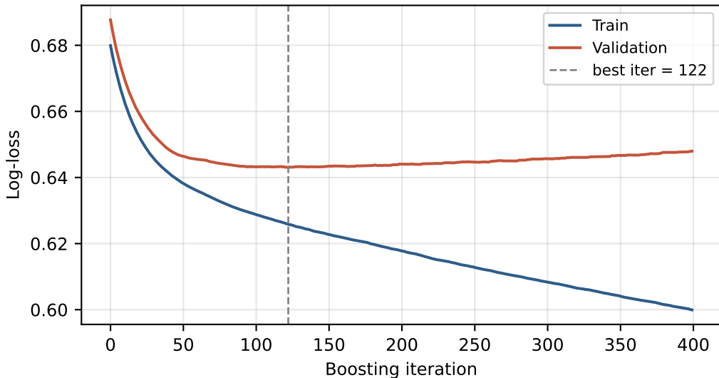
XGBoost training curve
