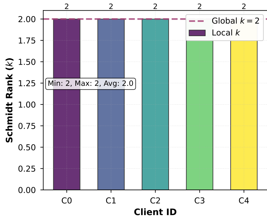
A. Local Schmidt Rank Distribution
