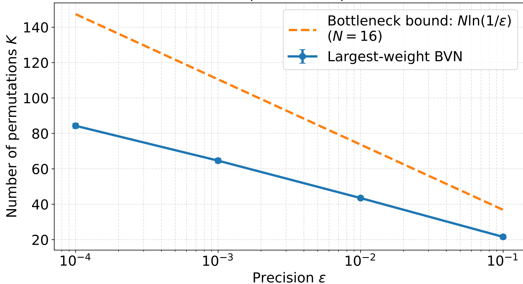
Term count vs. precision (4 qubits, N = 16 )
