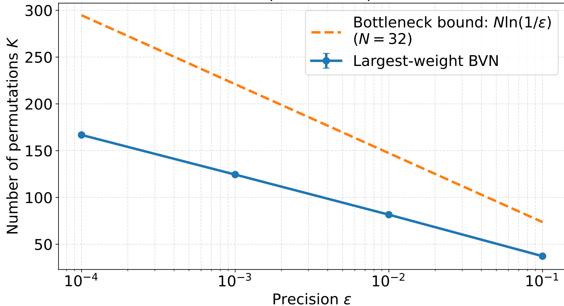
Term count vs. precision (5 qubits, N = 32 )
