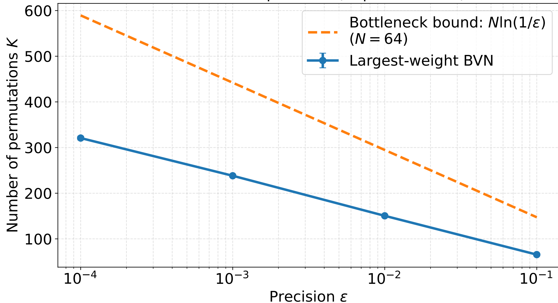
Term count vs. precision (6 qubits, N = 64 )
