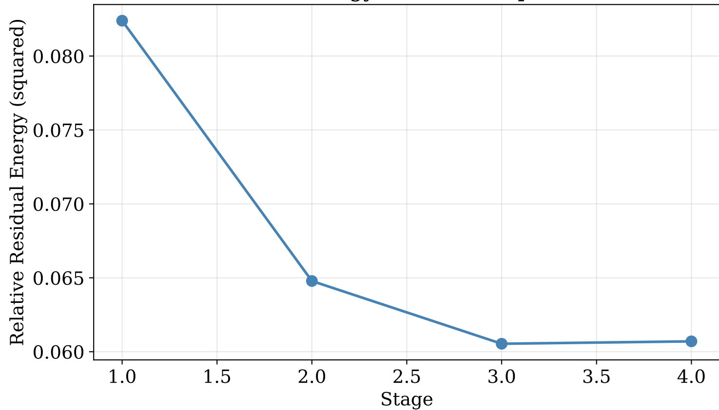
Residual Energy Reduction (qubits=6)
