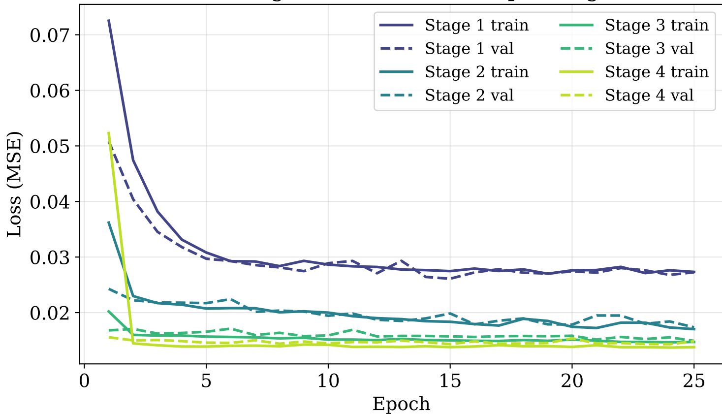
Training and validation loss per stage
