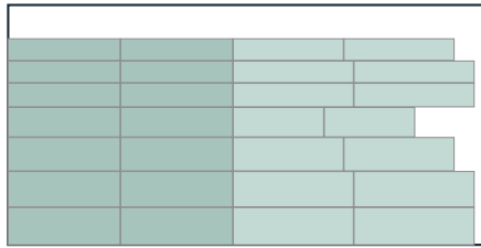
Sheet 8 — 12mm birch ply 79% used · 28 parts
