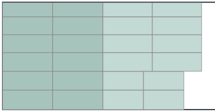
Sheet 7 — 12mm birch ply 88% used · 24 parts
