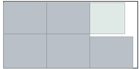
Sheet 9 — 6mm birch ply 90% used · 6 parts
