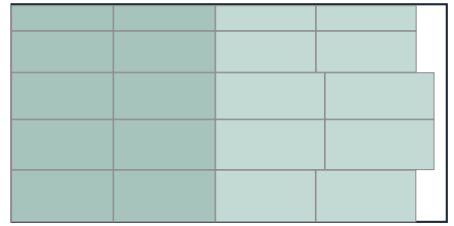
Sheet 6 — 12mm birch ply 93% used · 20 parts
