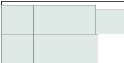
Sheet 10 — 1/4" birch ply 81% used · 7 parts
