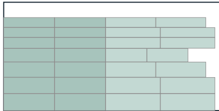
Sheet 8 — 1/2" birch ply 79% used · 28 parts
