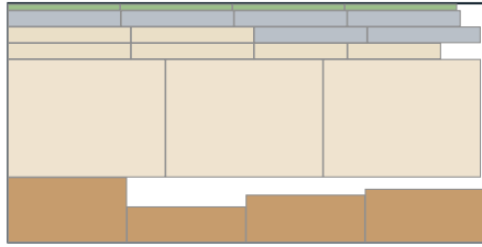
Sheet 2 — 11/16" birch ply 90% used · 23 parts
