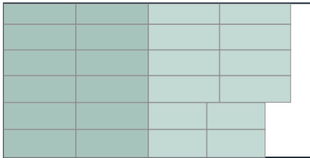
Sheet 7 — 1/2" birch ply 88% used · 24 parts
