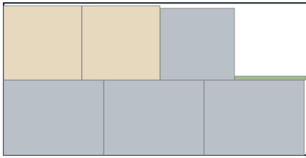
Sheet 4 — 11/16" birch ply 85% used · 7 parts
