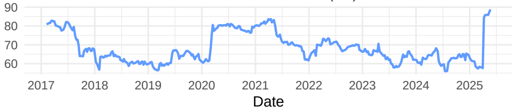
Total Connectedness Index (TCI)
