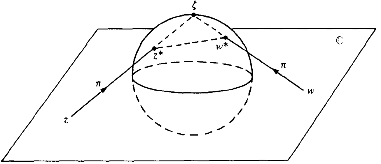
Figure 2.1: Stereographic projection.
