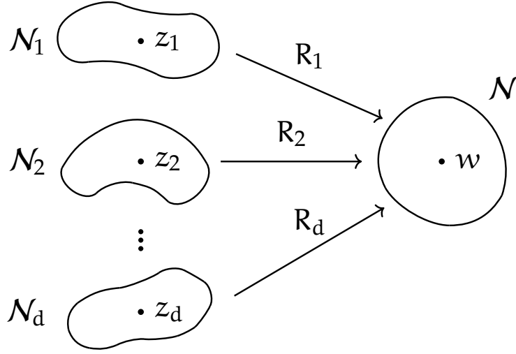
Figure 2.3: Bijective restrictions of R for a non-critical value w .
