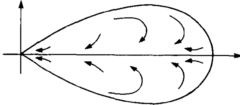
Figure 6.8: The dynamics on a petal.
