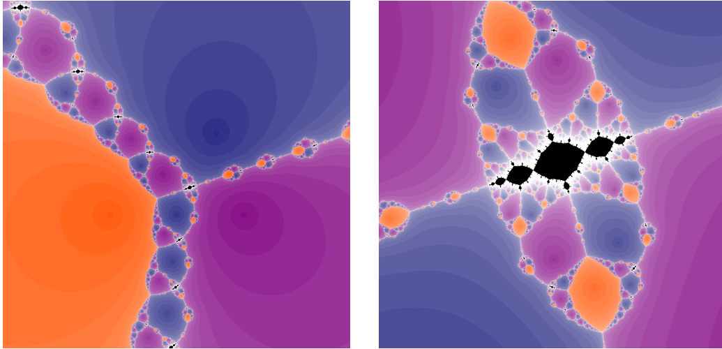
Figure 14: Left: the phase plane of Newton's method of the polynomial P(z) = z(z - 1)(z - a) with a chosen appropriately. Right: a zoom in which we see one of the sets of bad initial conditions. In this concrete case, it consists of the basin of attraction of a periodic orbit of period 2.
