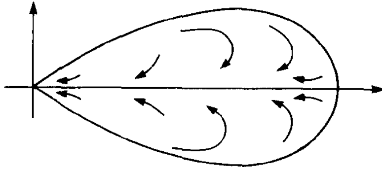
Figure 6.8: The dynamics on a petal.
