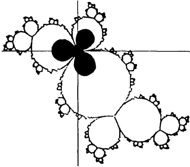
Figure 6.10: z \mapsto e^{2\pi i/3}z + z^2 .
