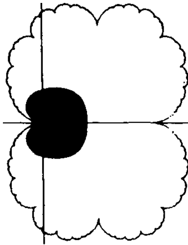
Figure 6.6: Julia set of z \mapsto z - z^2 .
