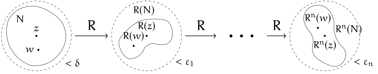
Figure 3.1: Equicontinuity for the family \mathcal{F} = \{R^n\}_{n \in \mathbb{N}} .
