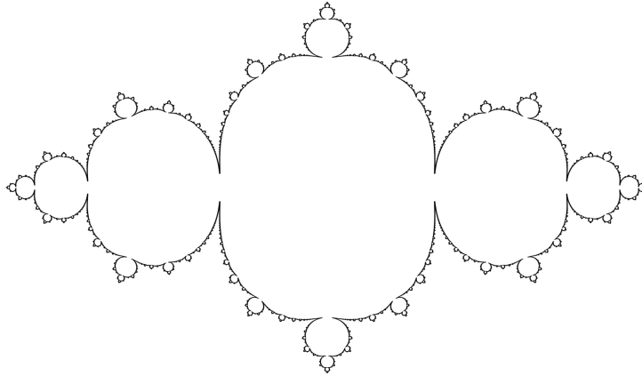
Figure 6.1: Julia set of z \mapsto z^2 - z .
