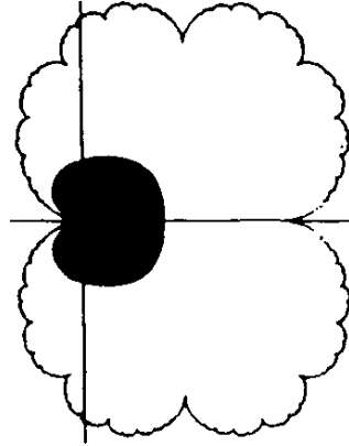
Figure 6.6: Julia set of z \mapsto z - z^2 .
