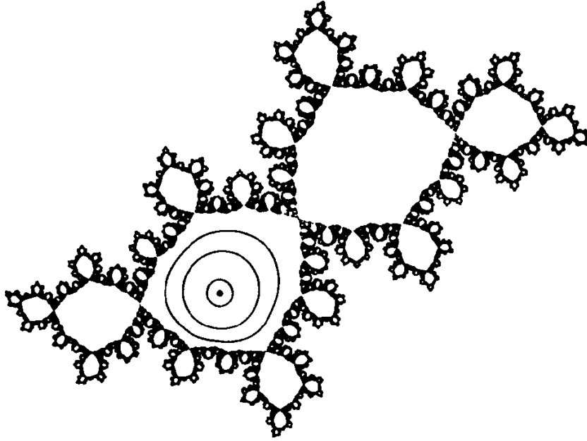
Figure 7.1: z \mapsto \lambda z + z^2 , \lambda = \exp(\pi i(\sqrt{5} - 1)) .
