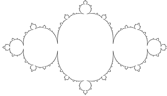
Figure 6.1: Julia set of z \mapsto z^2 - z .
