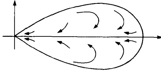
Figure 6.8: The dynamics on a petal.
