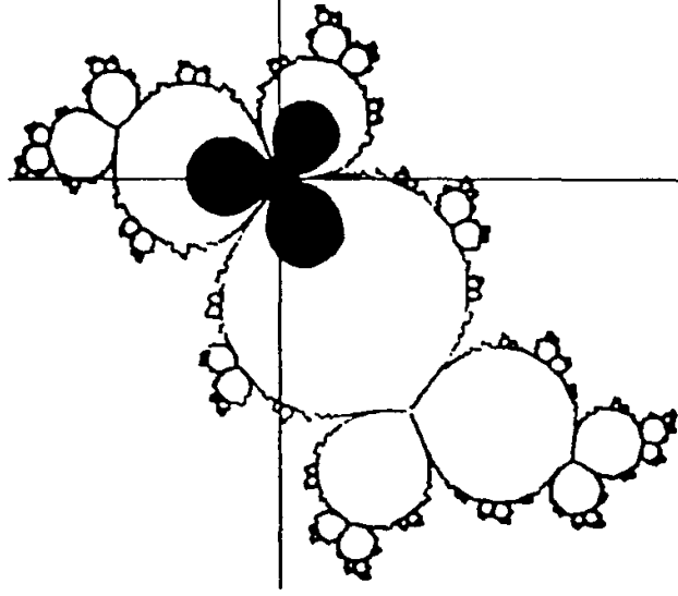
Figure 6.10: z \mapsto e^{2\pi i/3}z + z^2 .
