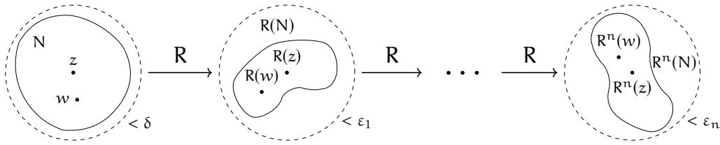
Figure 3.1: Equicontinuity for the family \mathcal{F} = \{R^n\}_{n \in \mathbb{N}} .
