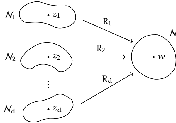
Figure 2.3: Bijective restrictions of R for a non-critical value w .
