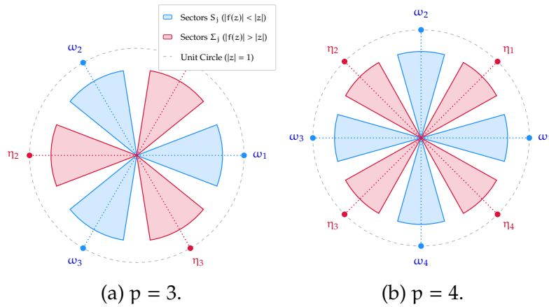
Figure 6.3: Alternating attracting and repelling sectors for a rationally indifferent point
