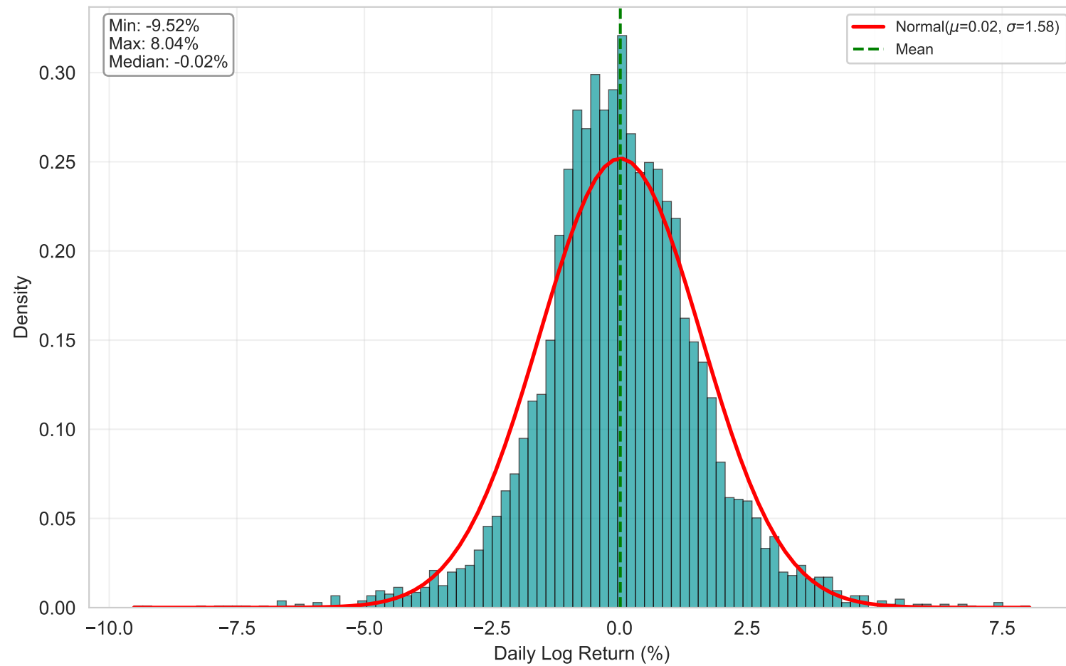
Soybean Oil Skew=-0.10, Kurt=2.30
