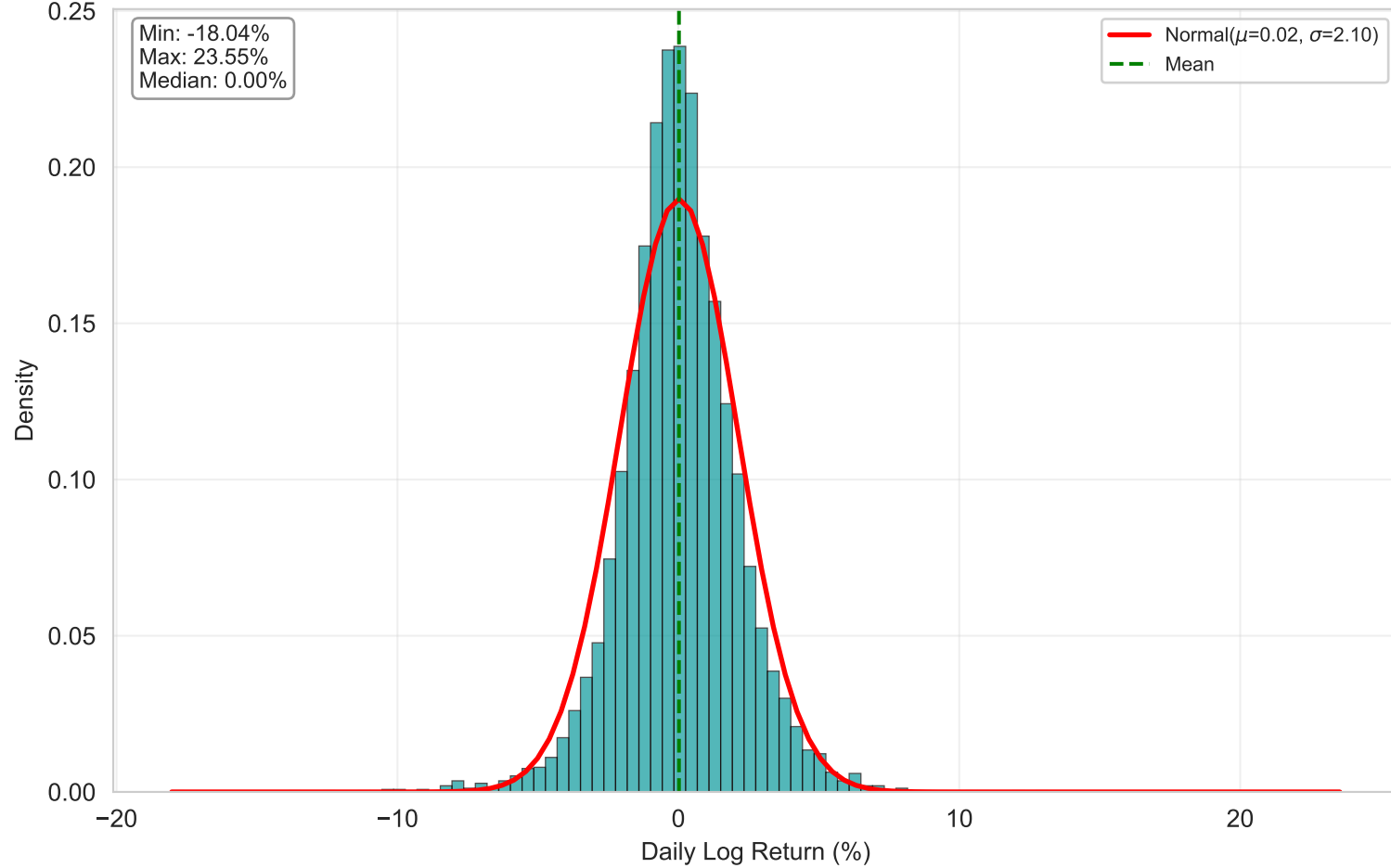
Sugar Skew=-0.03, Kurt=5.97
