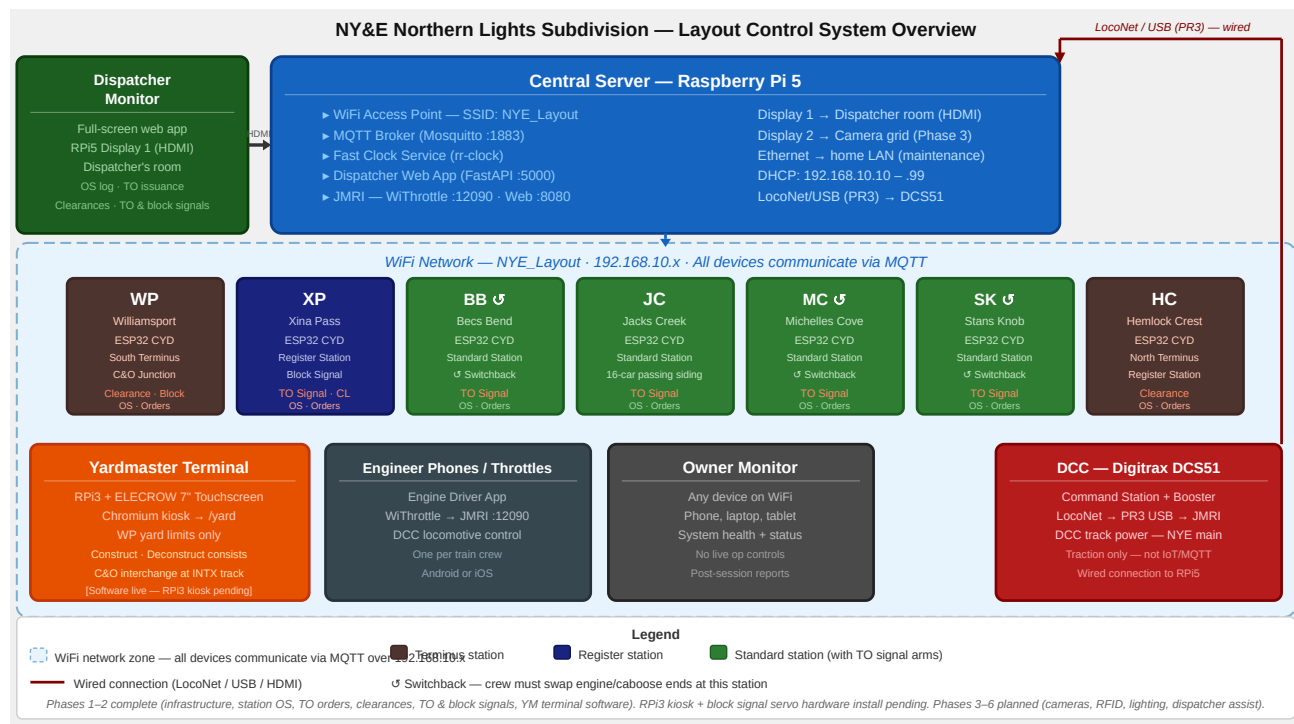
Figure 3. System block diagram — RPi5 server, MQTT broker, CYD station units, dispatcher web app.
