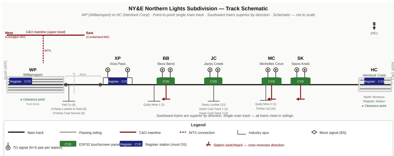
Figure 1. Track schematic, WP to HC — Northern Lights Subdivision.
