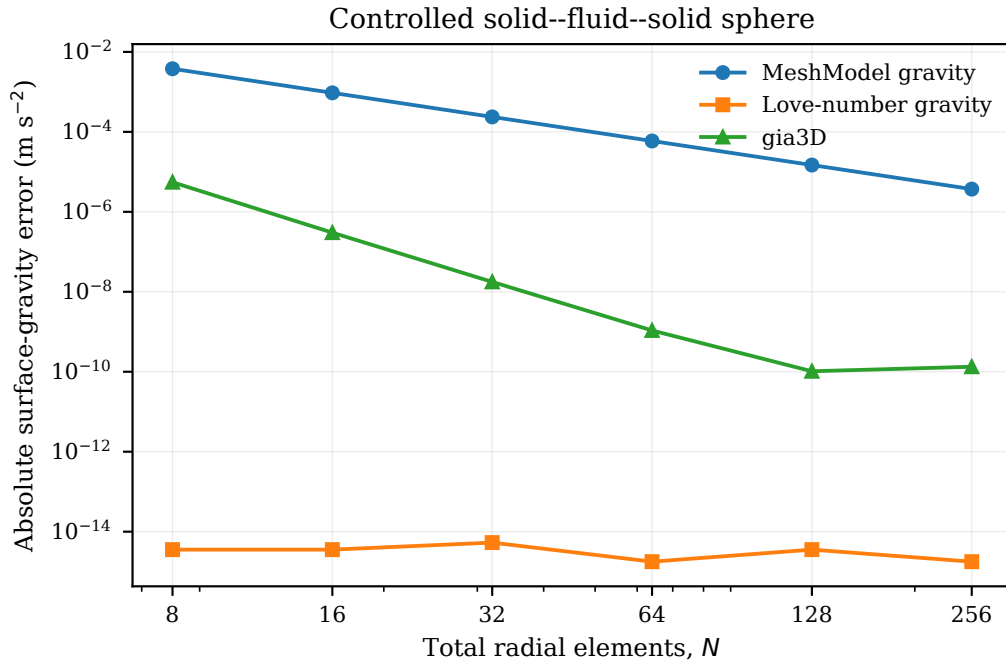
Figure 1: Absolute surface-gravity error for the controlled solid–fluid–solid density profile. The legacy curve is the existing MeshModel value, the orange curve is the gravity used by the Love-number module, and the green curve is the pinned gia3D reference.
