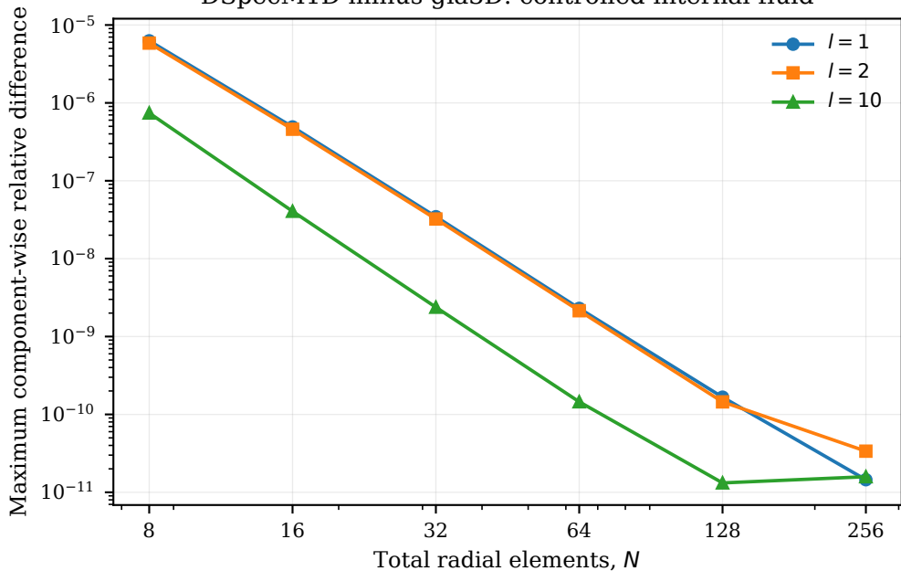
DSpecM1D minus gia3D: controlled internal fluid
