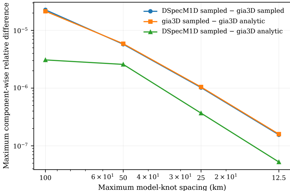
Isotropized no-ocean PREM, radial step 0.0025
