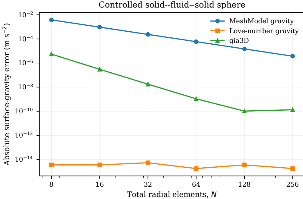
Figure 1: Absolute surface-gravity error for the controlled solid–fluid–solid density profile before the main-library correction. The legacy curve is the pre-correction MeshModel value, the orange curve is the former private Love-number integration, and the green curve is the pinned gia3D reference. The historical data are retained unchanged.
