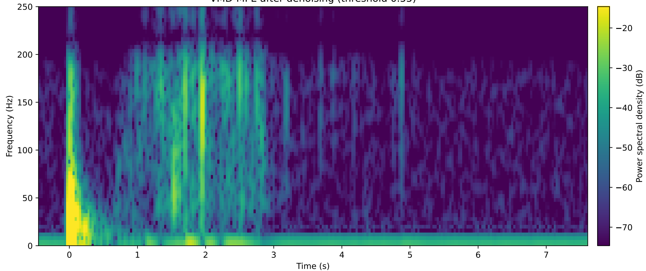
VMD-MPE after denoising (threshold 0.55)
