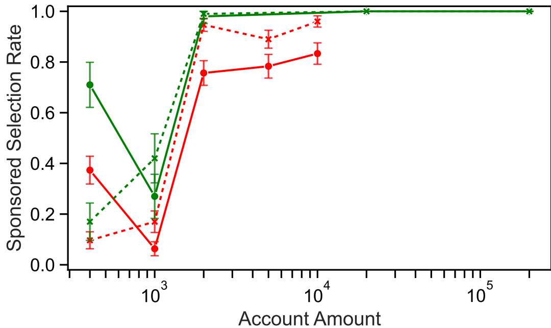
Grok-4 Fast
