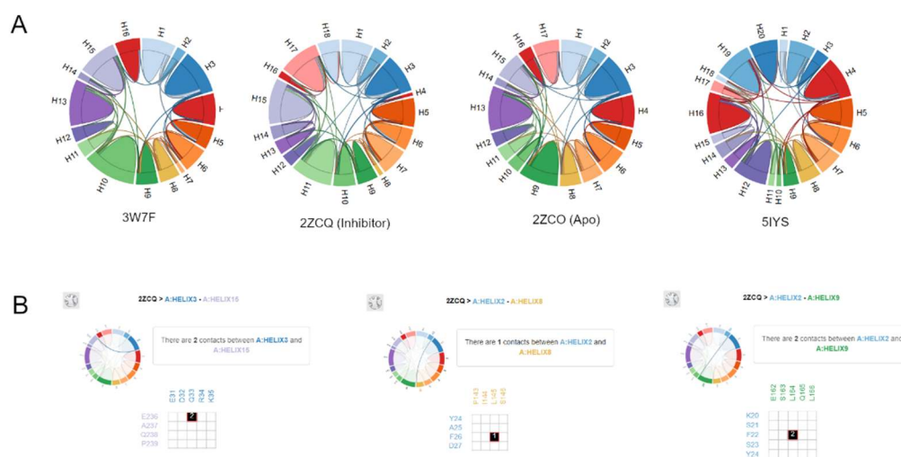
Figure S1 Helix Interaction Dynamics. (A) Chord diagrams representing inter-helix contacts for CrtM structures: Holo (3W7F), Inhibitor-bound (2ZCQ), Apo (2ZCO), and Holo (5IYS). The thickness of chords represents contact density; the Apo form exhibits a notable reduction in connectivity involving Helix-2 compared to ligand-bound states. (B) Detailed contact matrices for the 2ZCQ structure highlighting specific stabilizing interactions: Helix-3(Q33)–Helix-15(E236), Helix-2(F26)–Helix-8(L145), and Helix-2(F22)–Helix-9(L164). These interactions lock the binding cavity in the active conformation.
