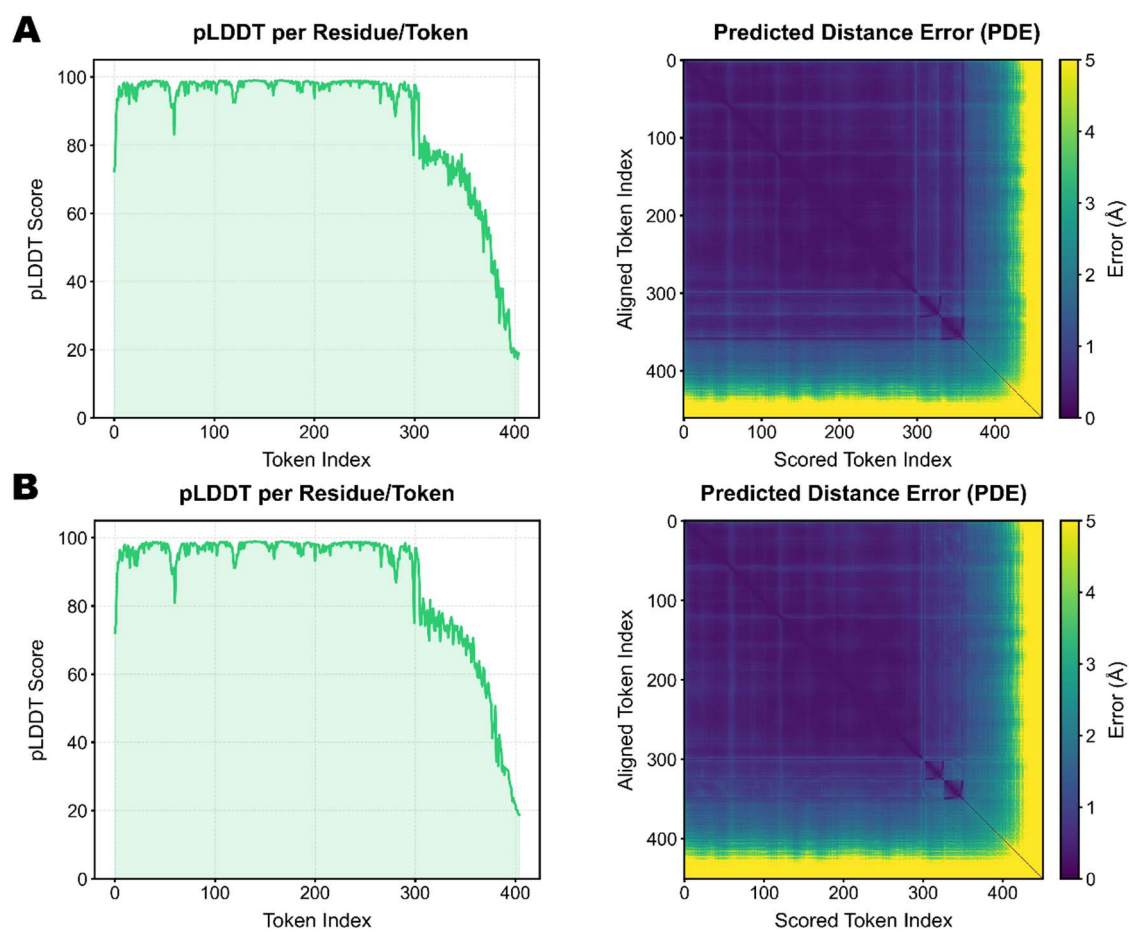
Figure S5. OpenFold prediction confidence metrics for PSY substrate complexes.
