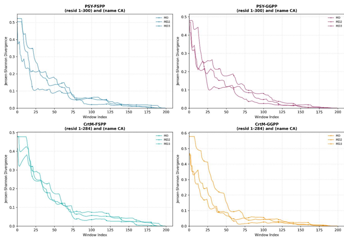
Figure S2. Convergence Analysis shows a plateau in the plot occurring between window times 50 and 75.
