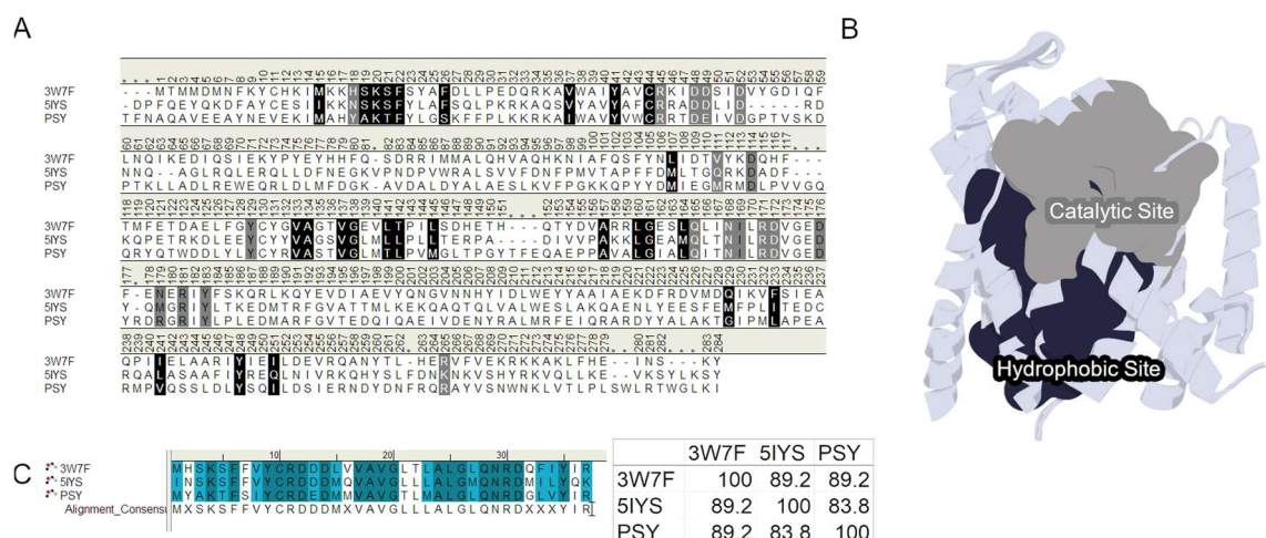
Figure S3. (A) Sequence alignment of CrtM (3W7F and 5IYS) and PSY (CrtB from Euglena gracilis without the irregular region sequence, accession No BAU24764.1). Residues corresponding to the ligand-binding site are highlighted, with catalytic residues shaded in gray and the hydrophobic site marked in black. (B) Structural presentation of the Catalytic Site (gray clouded area) and Hydrophobic Site (black clouded area). (C) The Binding cavity sequences similarity percentage.
