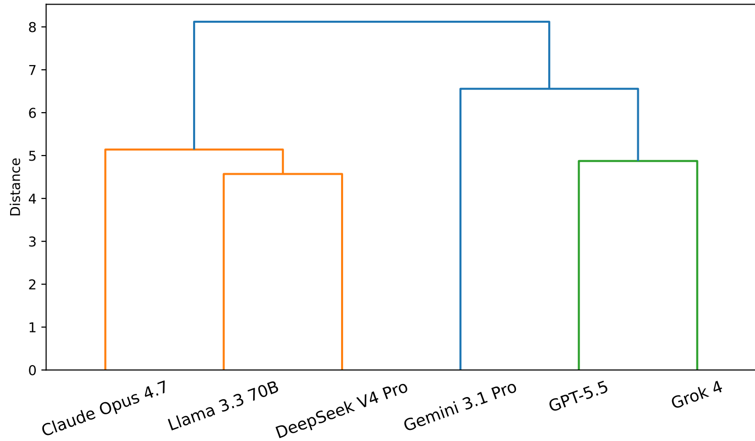
Cross-task model clustering — Ward linkage on z-scored 15-dim profiles
