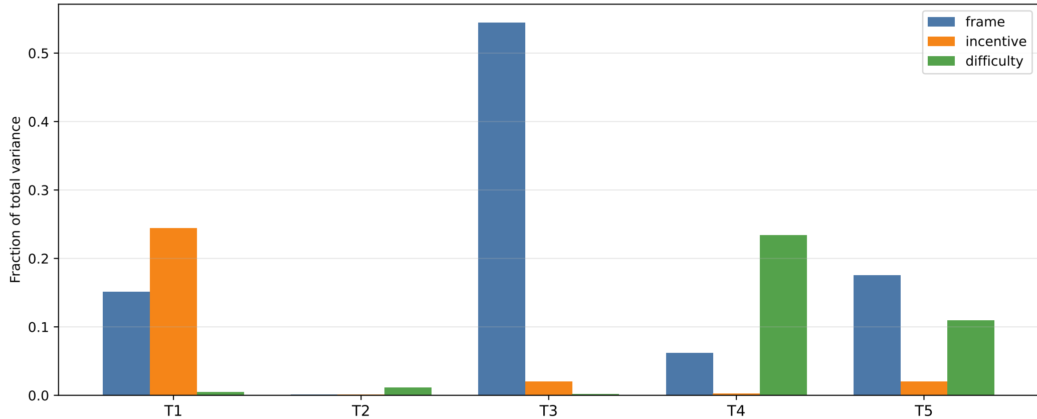
Variance decomposition: per-axis between-group share of total variance, per task ( \eta^2 -style; residual = within-cell variance + interaction effects)
