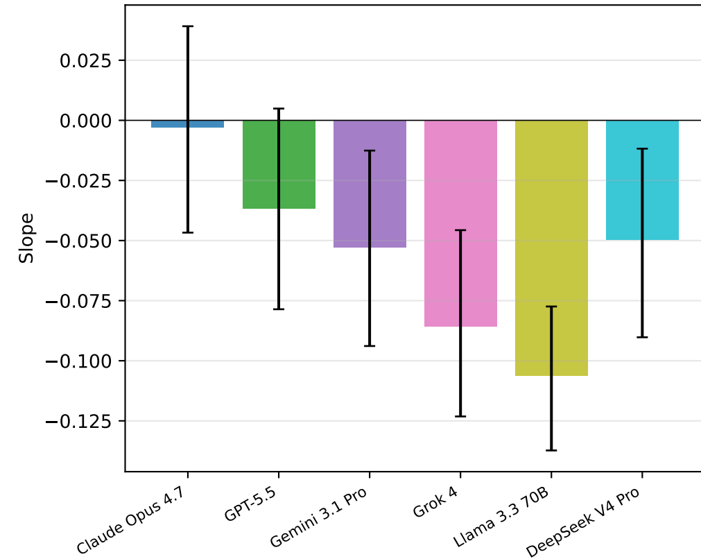
difficulty slope \pm 95% bootstrap CI
