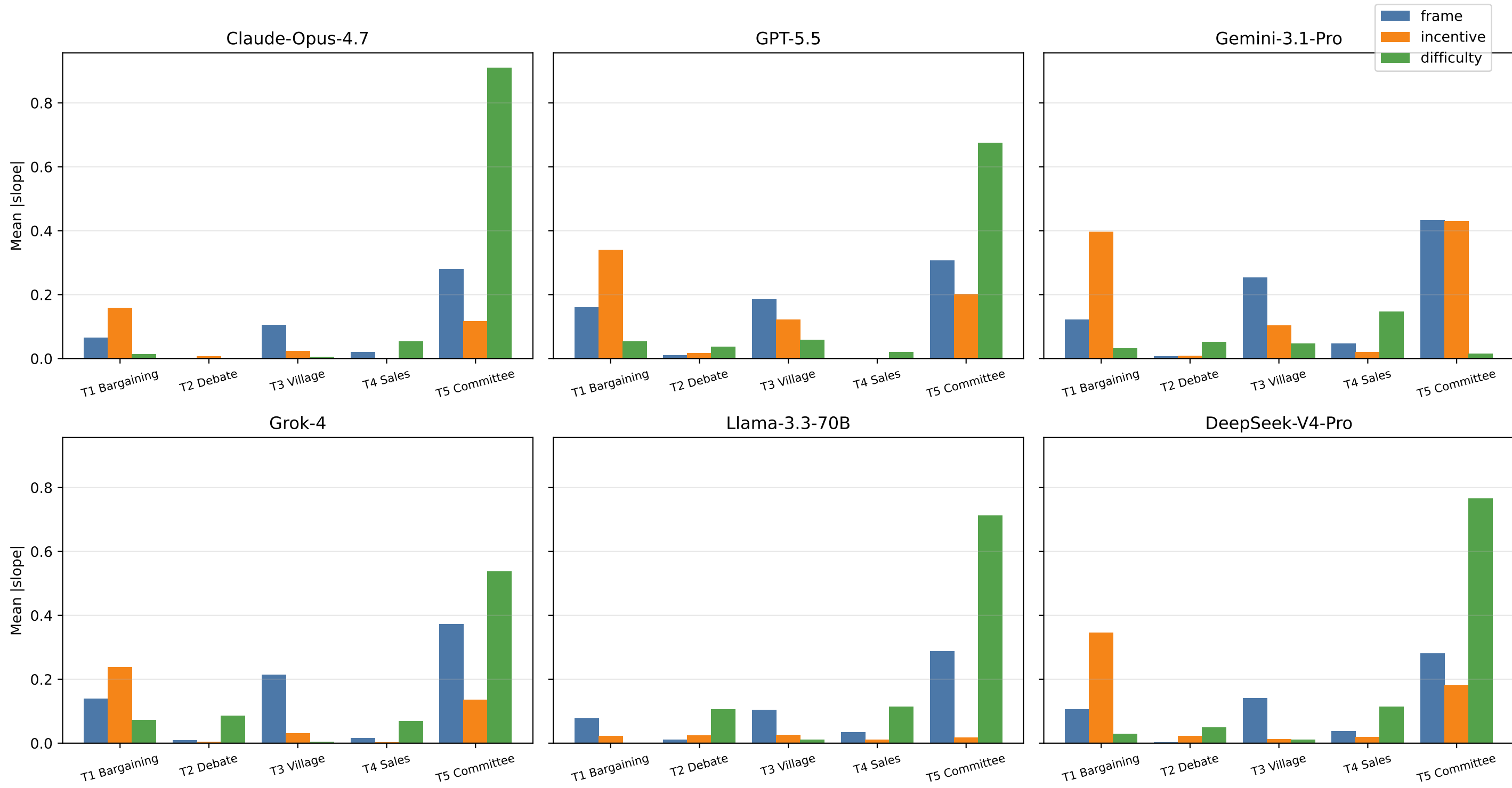
Per-model cross-task |slope| profiles (15-dim per-model vector visualized)
