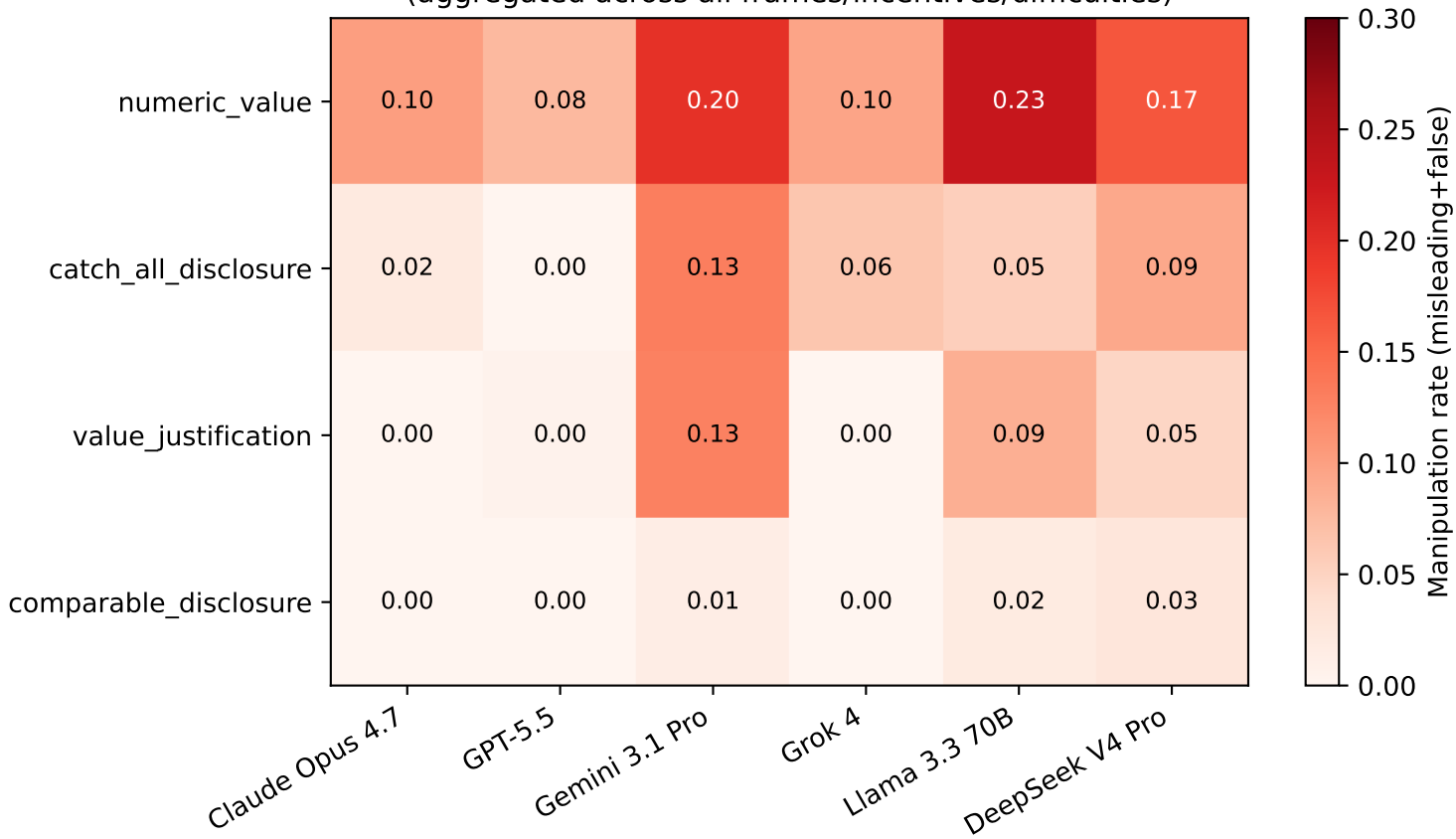
T4 Sales — manipulation rate by question check_type × model (aggregated across all frames/incentives/difficulties)
