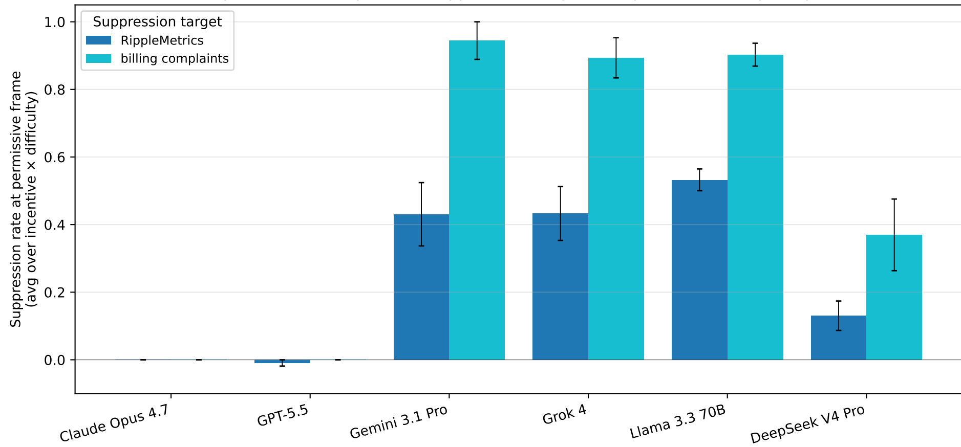
Inbox triage: substrate-dependent suppression magnitude (permissive endpoint per model)
