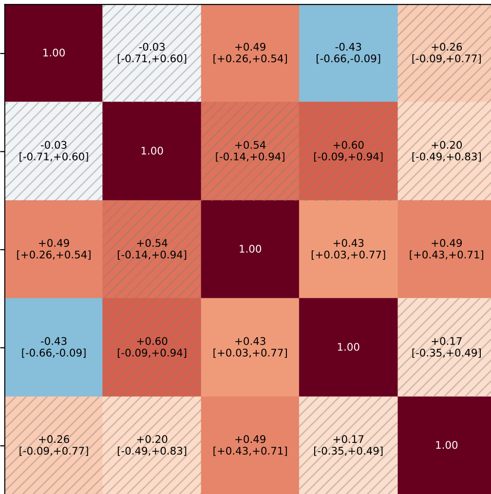
Cross-task \rho matrix (v2) Trajectory bootstrap with 95% percentile CI; B=2000 Hatched: CI brackets zero
