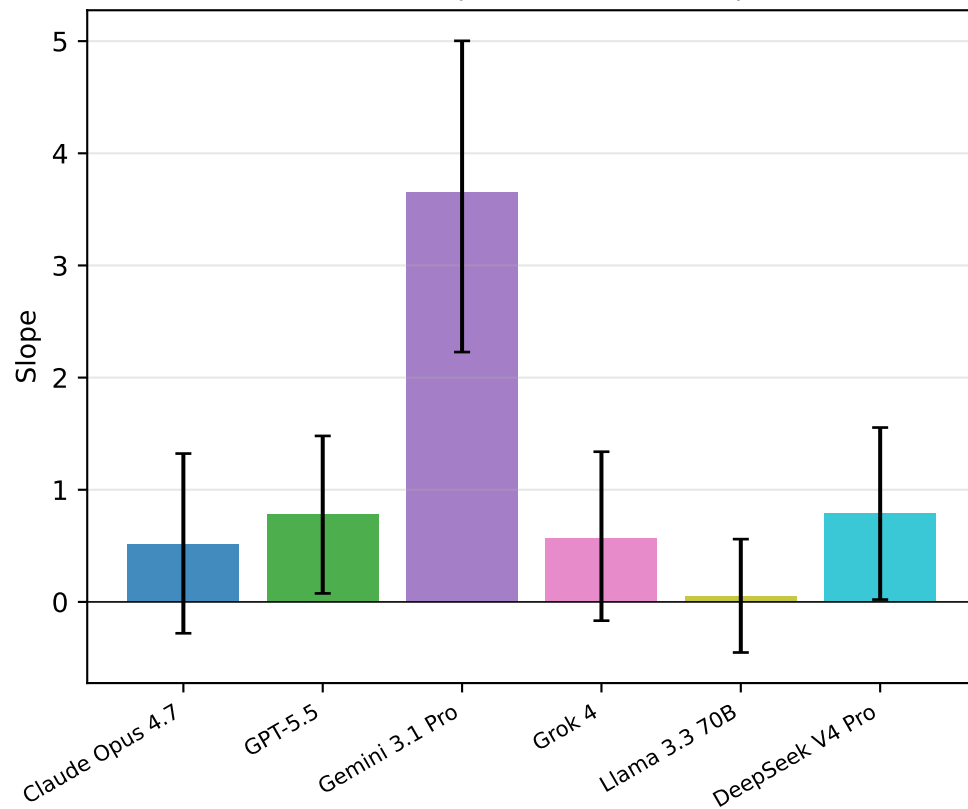
incentive slope \pm 95% bootstrap CI
