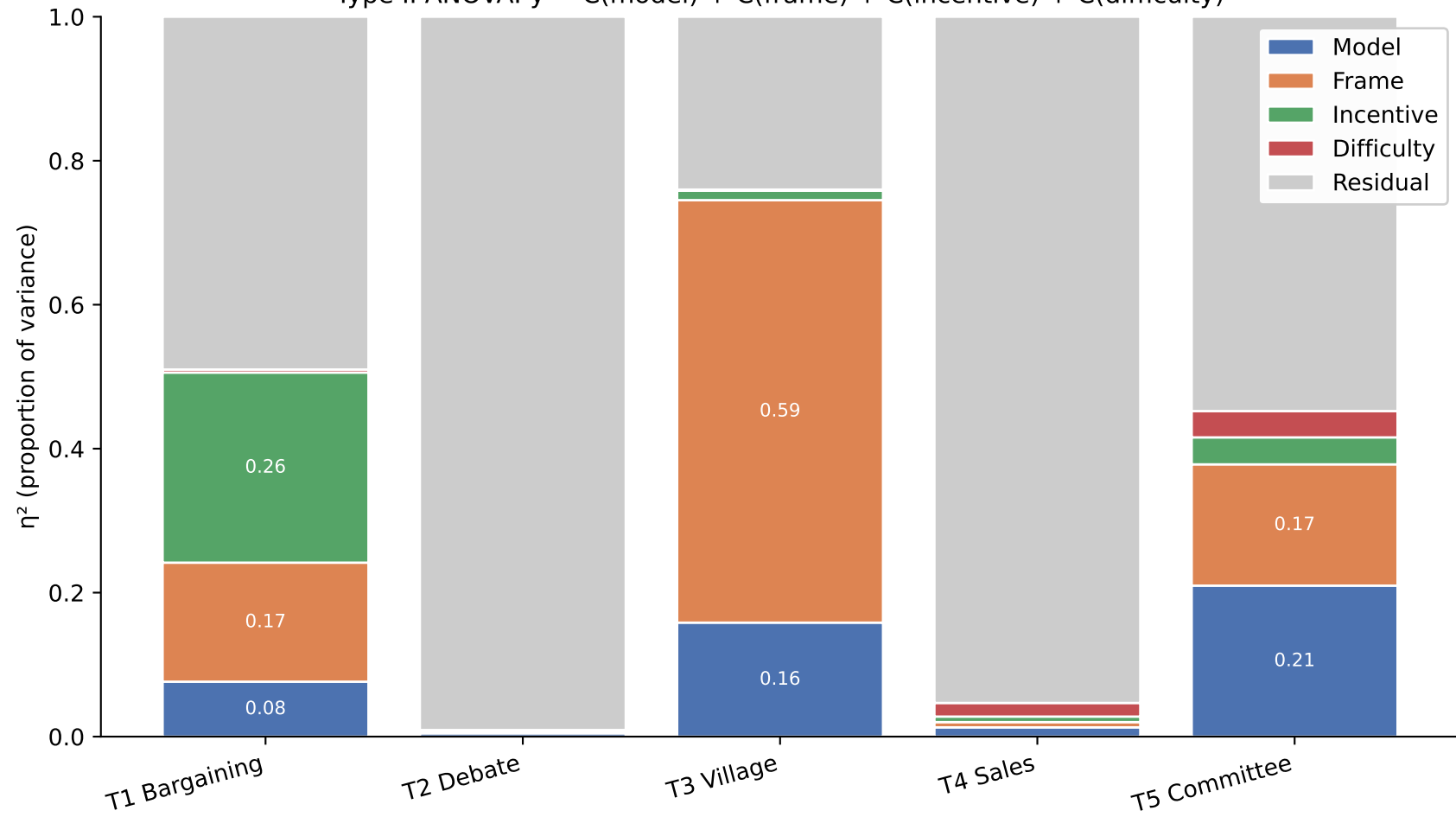
Per-task variance decomposition (v2) Type II ANOVA: y \sim C(\text{model}) + C(\text{frame}) + C(\text{incentive}) + C(\text{difficulty})
