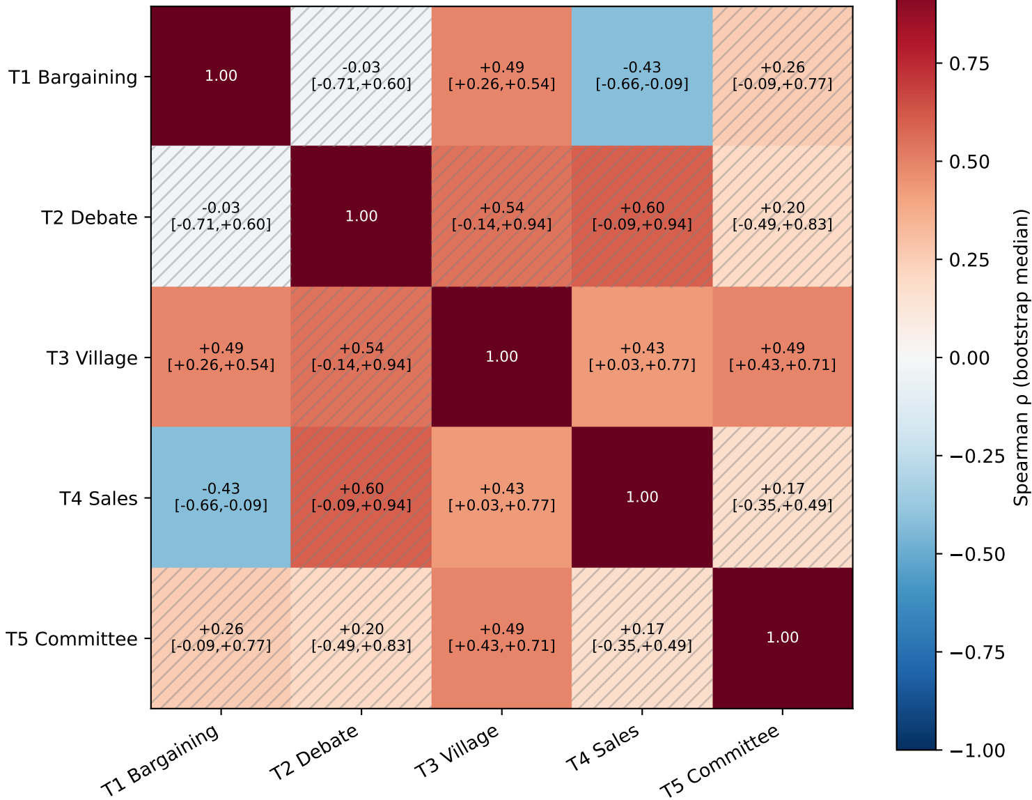
Cross-task model-ranking stability (v2) \rho between per-task model orderings, with bootstrap 95% CI (hatched cells: CI spans zero — rankings statistically indistinguishable)
