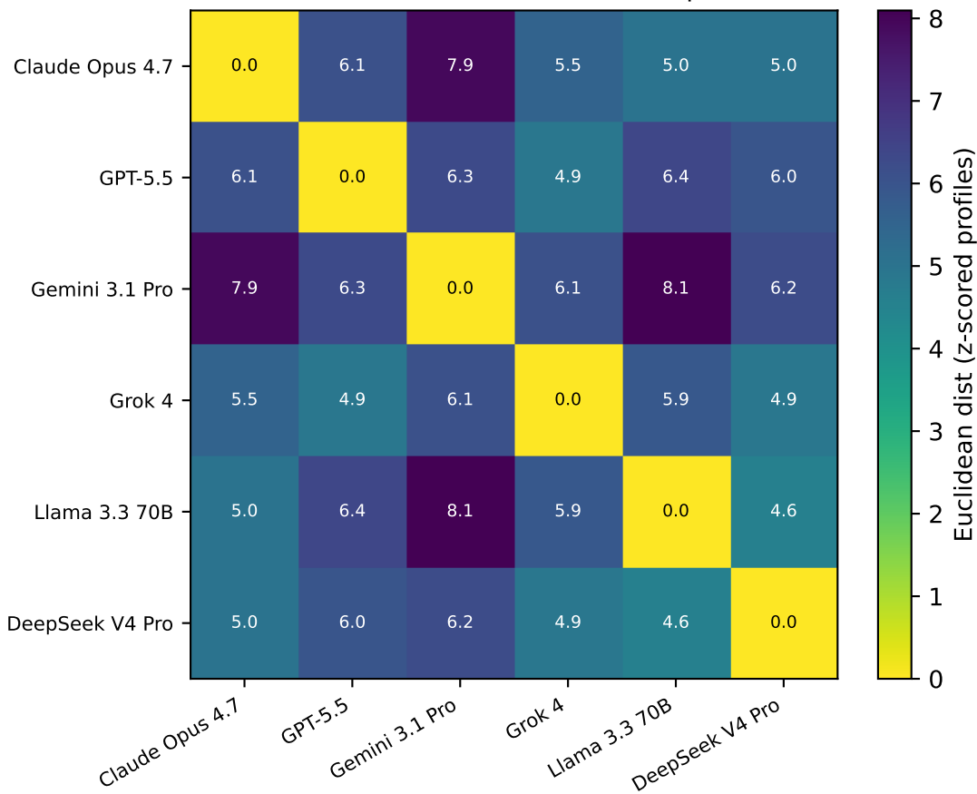
Cross-task model distance matrix (15-dim profile, z-scored)
