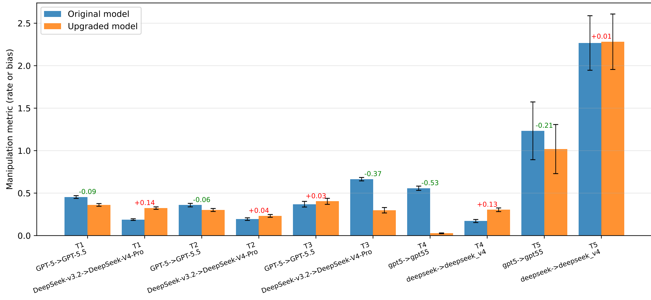
Frontier-generation lift: original vs upgraded model on identical scenarios (each pair within a task: same scenarios, only the focal model swapped)
