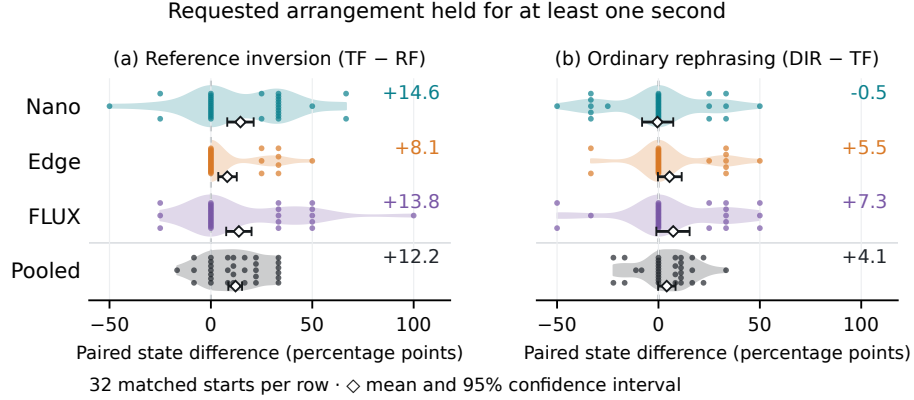
Figure 1: Wording effects across 32 physical starts. Dots show each start’s average outcome difference. Diamonds and bars show means and 95% intervals. Positive TF - RF favors target-first wording. Wider sections indicate more starts with similar effects.
