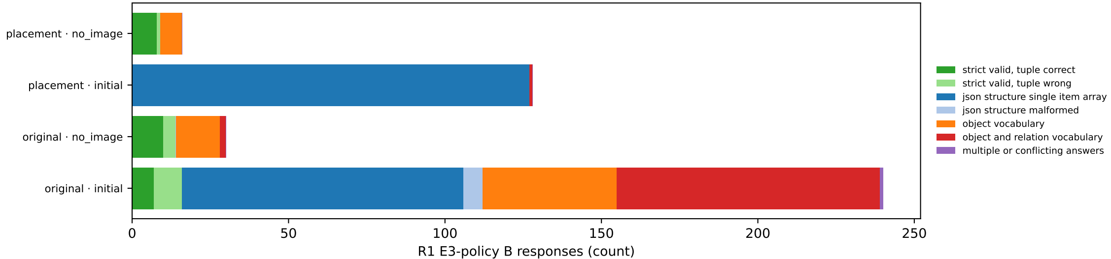
Edge R1 free-generation B responses on S1/S3/S4: strict validity and format-failure classes (no repair)
