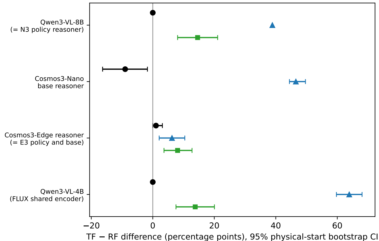
Where the wording gap appears
