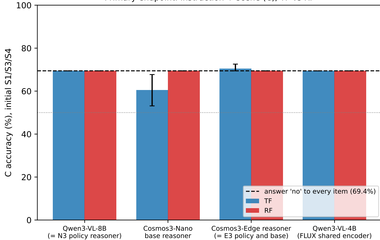
Primary endpoint: instruction + scene (C), TF vs RF
