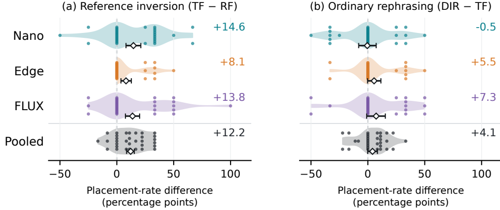
Figure 1: Wording effects across 32 starts per row. Each dot’s horizontal position shows that start’s average placement-rate difference; vertical offsets only separate dots. Wider shading indicates more starts with similar effects. Diamonds and bars show means and 95% confidence intervals. Positive values favor TF in (a) and DIR in (b).
