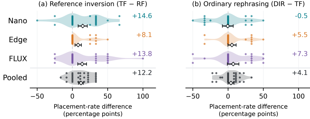
Figure 1: Wording effects on stable placement: the requested arrangement holds for at least one second. Each row shows 32 physical starts. Dots show each start’s difference in stable-placement rate, averaged over goals (and models for Pooled). Horizontal positions are percentage-point differences; vertical offsets only prevent overlap. Shading is thicker where more starts have similar effects. Diamonds and bars show means and 95% confidence intervals. Positive values favor TF in (a) and DIR in (b).
