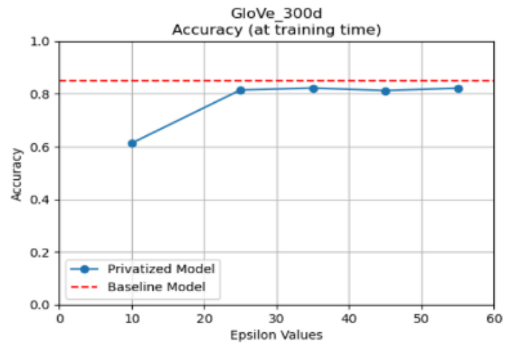
Figure 4.3: Accuracy vs \epsilon for Glove(300d) in Training Time
