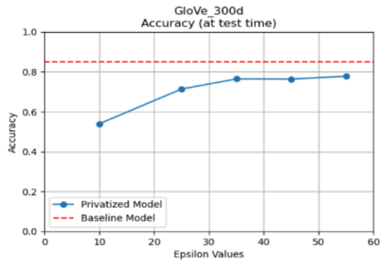
Figure 4.4: Accuracy vs \epsilon for Glove(300d) in Test Time
