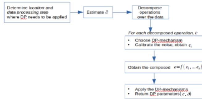
Figure 3.2: A step by step guide on how to incorporate DP in ML
