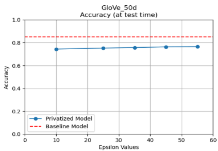
Figure 4.2: Accuracy vs \epsilon for Glove(50d) in Test Time
