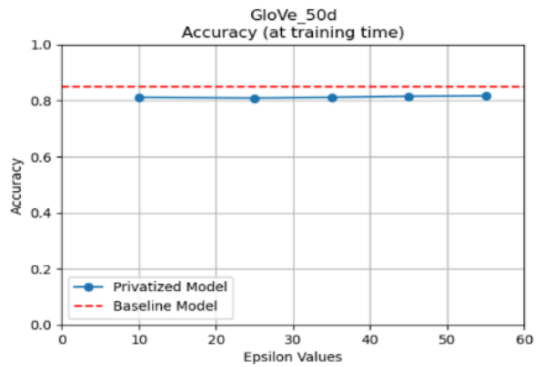
Figure 4.1: Accuracy vs \epsilon for Glove(50d) in Training Time
