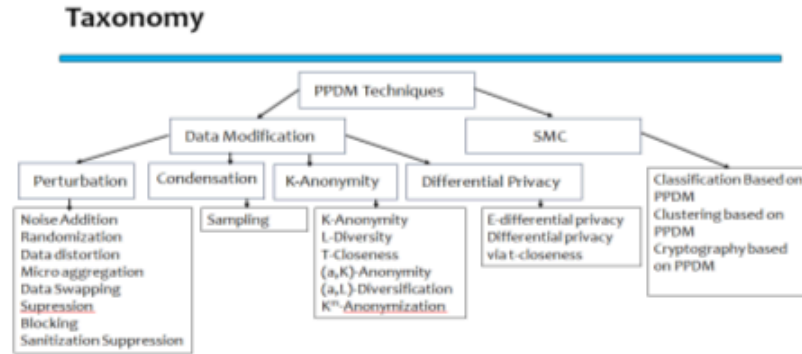
Figure 3.1: Taxonomy of PPDM Techniques
