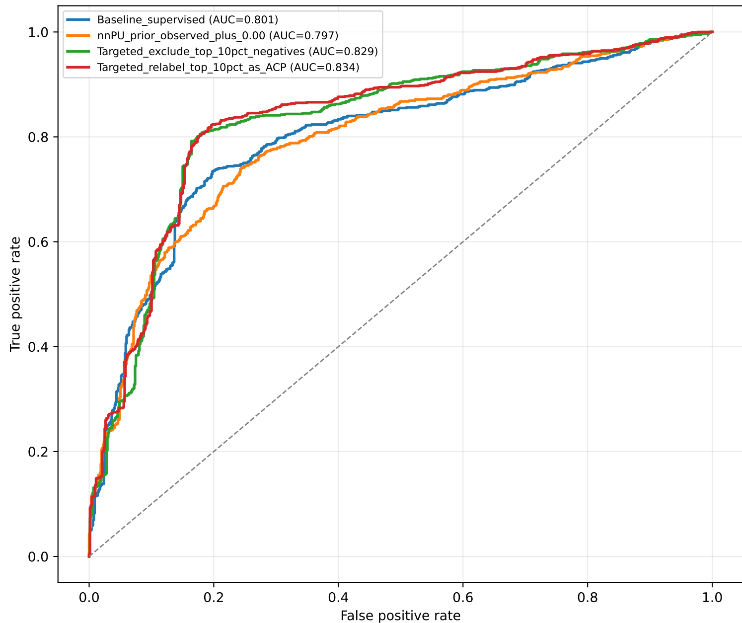
Pooled out-of-fold ROC curves
