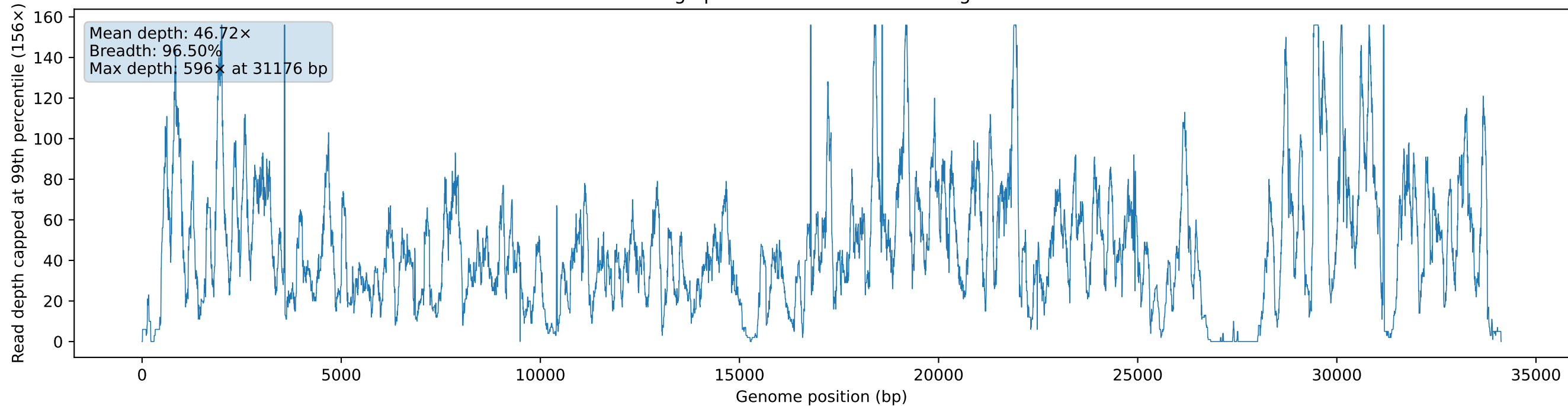
Coverage profile — Goat AdV-12-like genome
