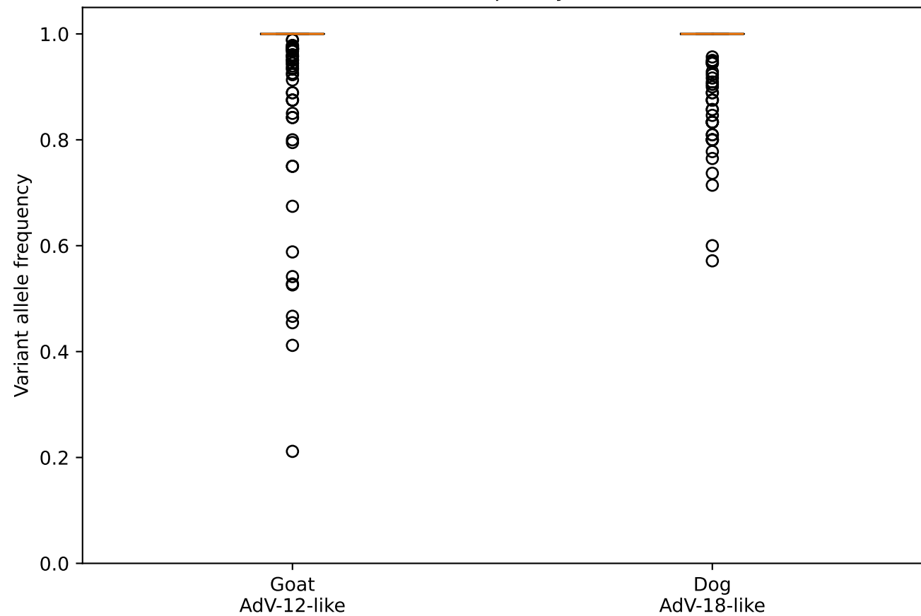
Variant allele frequency distribution
