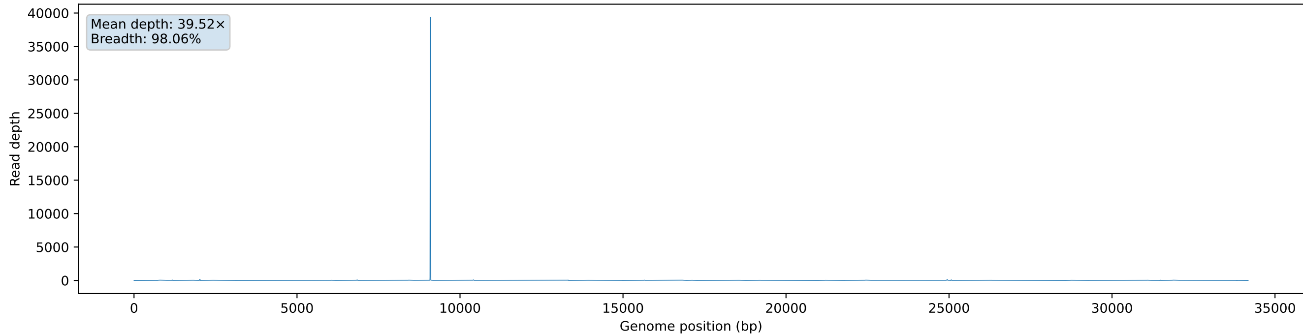
Coverage profile — Dog AdV-18-like genome
