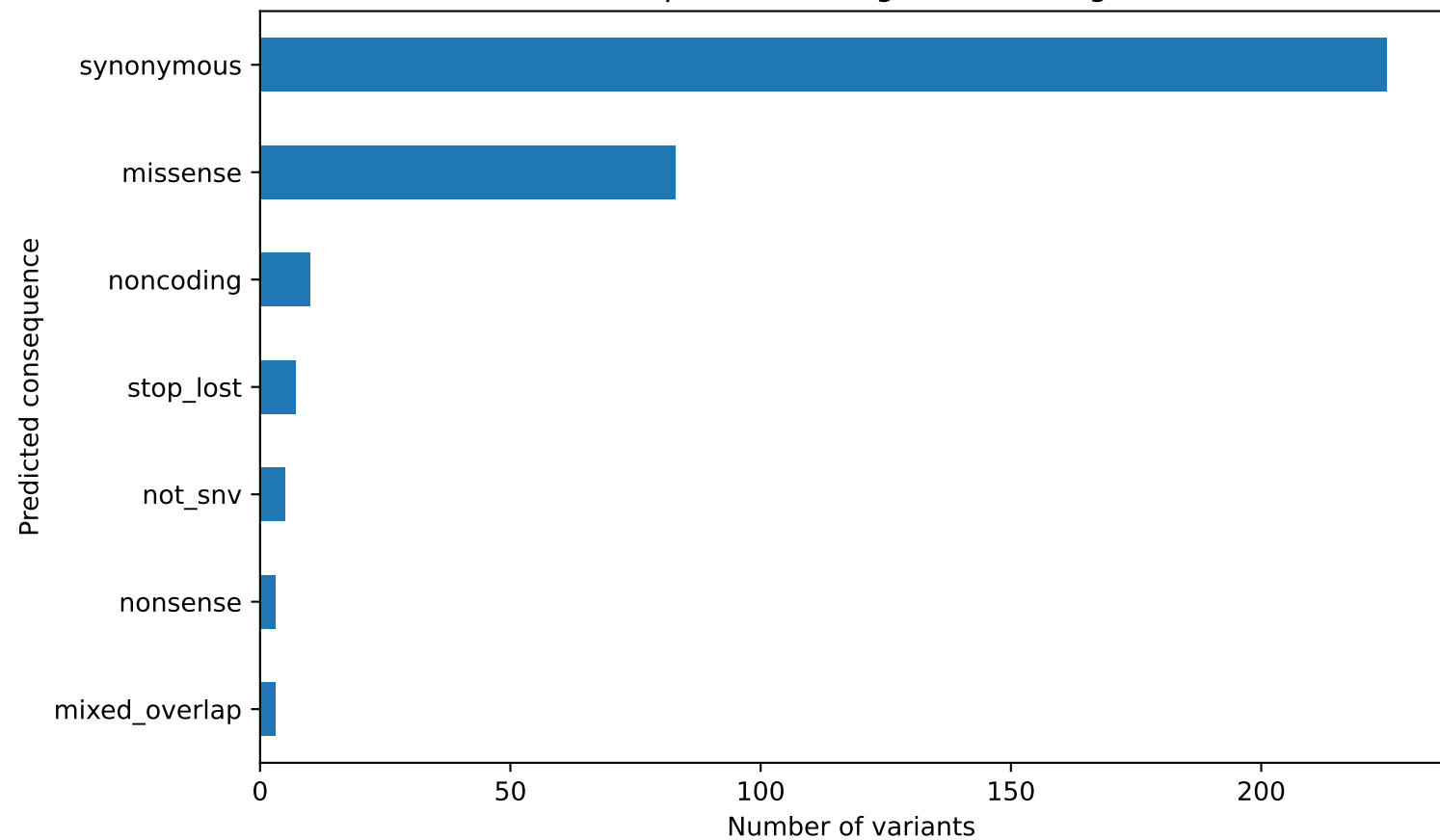
SNV consequences — Dog AdV-18-like genome
