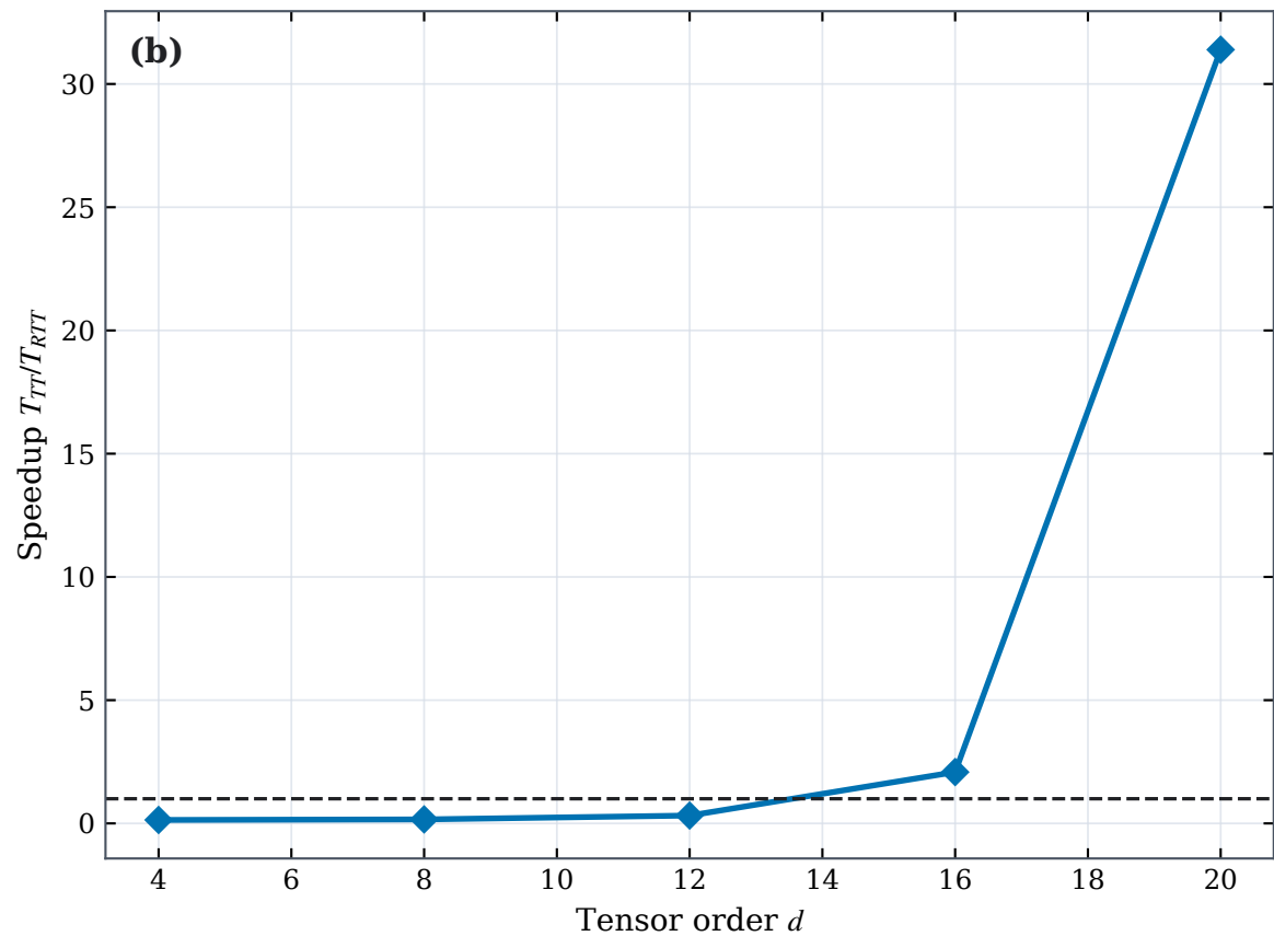
Measured speedup where dense TT-SVD is feasible
