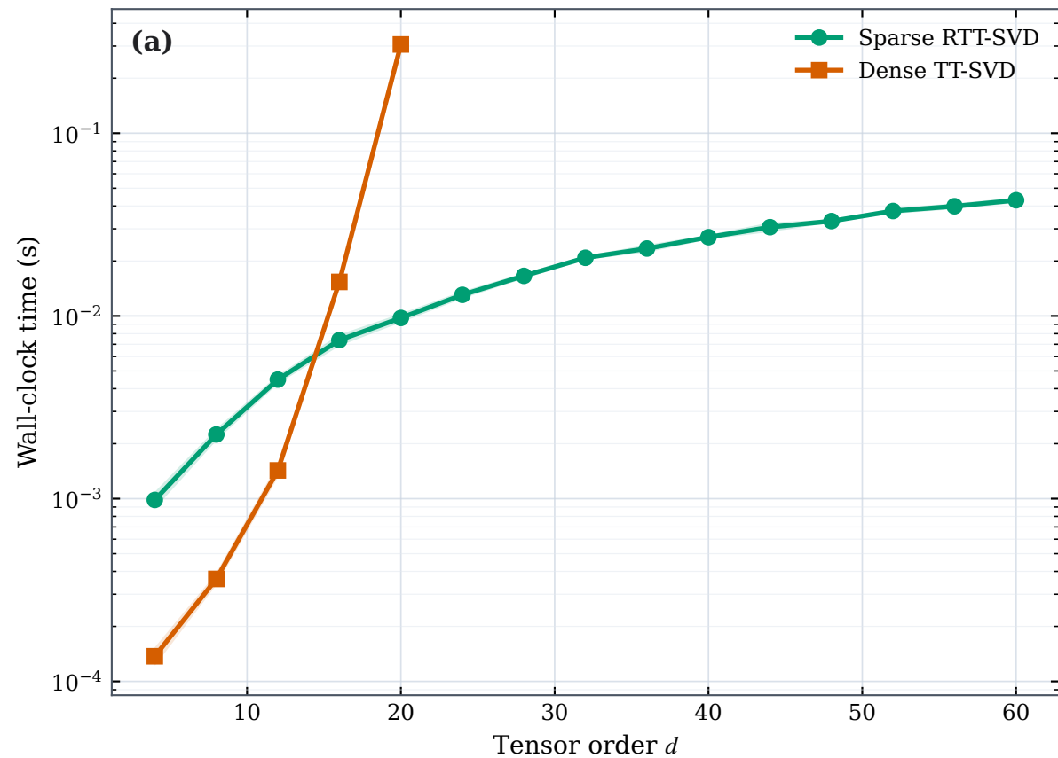
Runtime, N = 500 , n = 2
