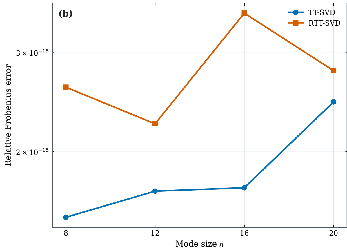
Exact-recovery check
